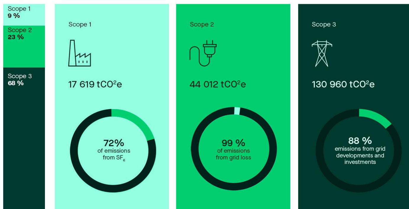
Figure 6: GHG-emissions
