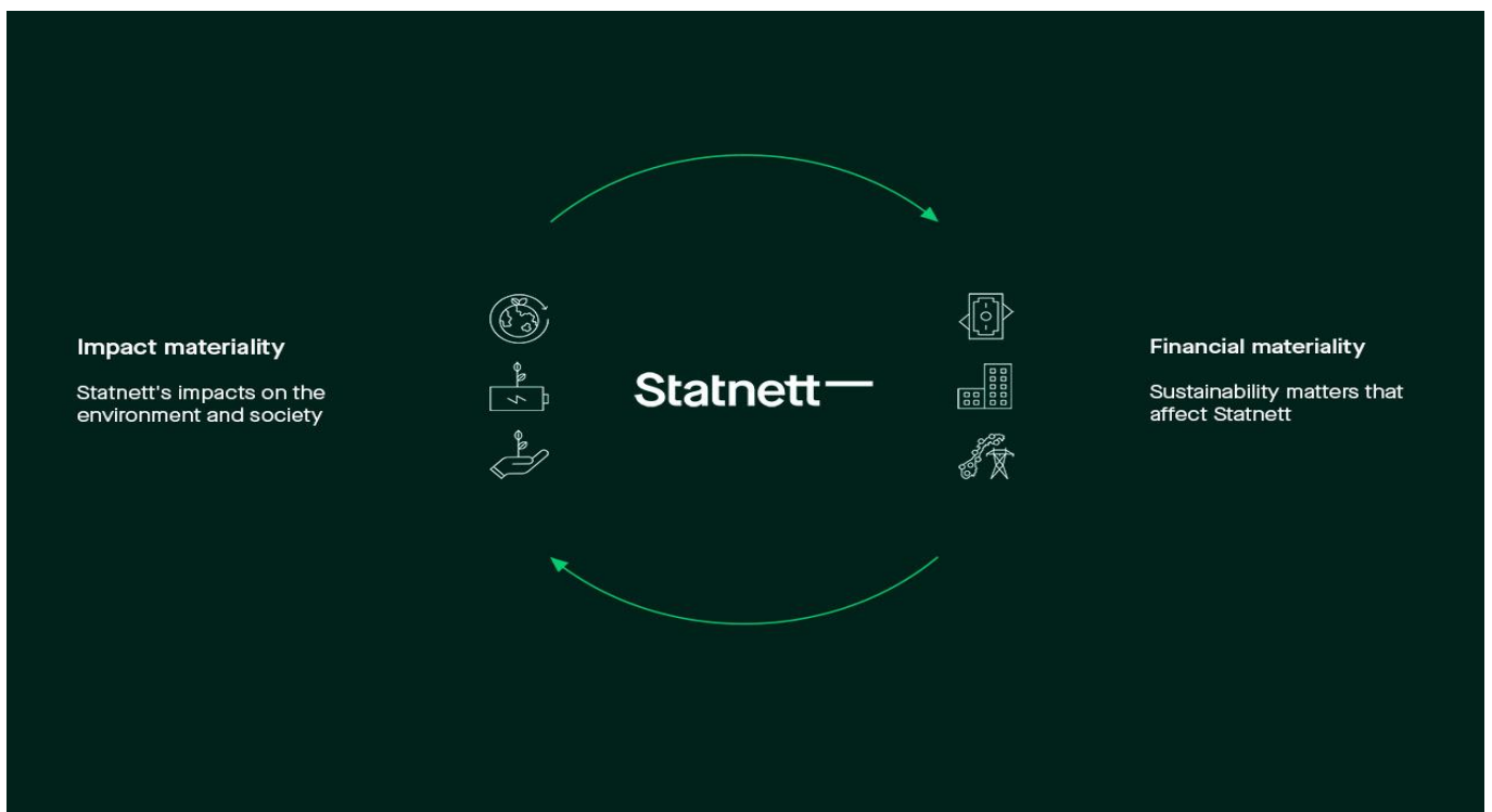
Figure 2: Double materiality
